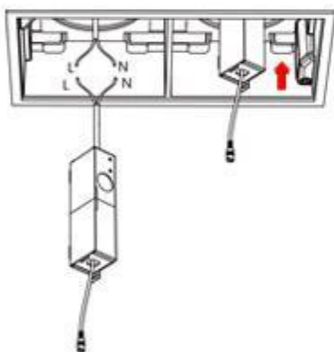
4. wire the driver
